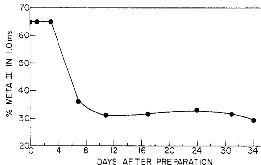
Figure 10. Meta-II production during the first msec as a function of age of the preparation. Frog rhodopsin in 2% digitonin, pH 6.5, 25°, bleached with a 2-msec flash from a Honeywell 65-C Stroboscoper through a Wratten 2E filter.
